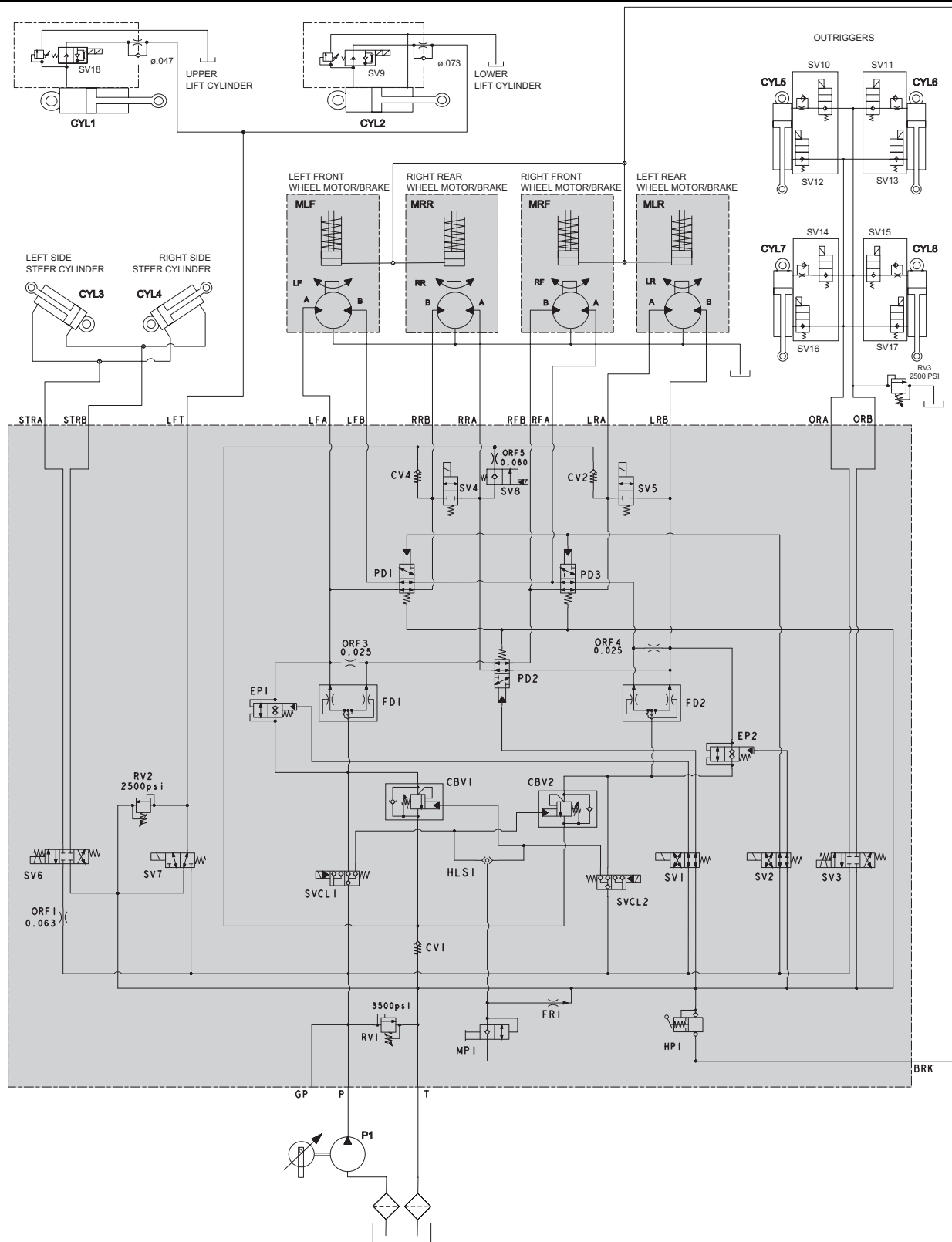
Figure 5-1: Hydraulic Schematic
