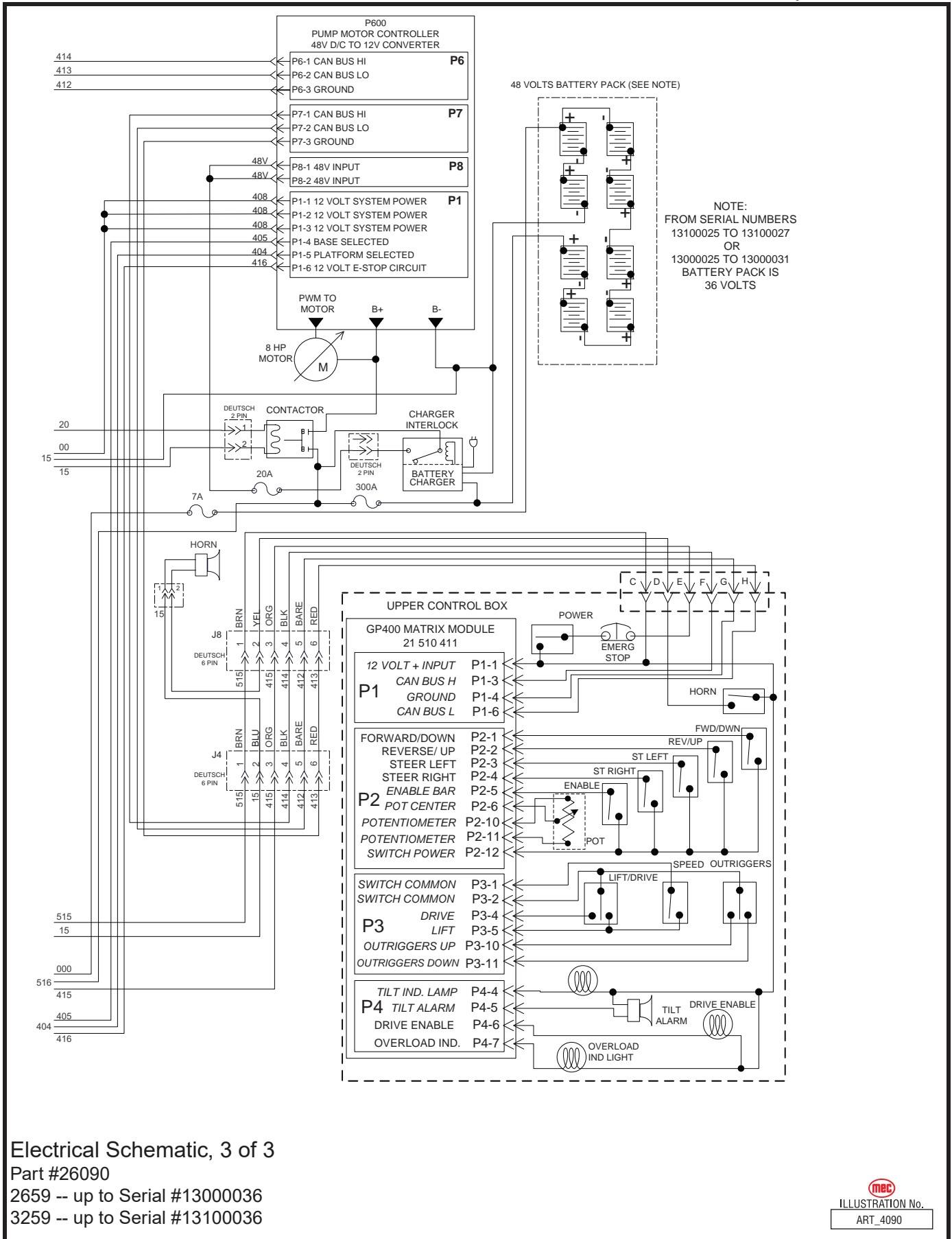
Figure 5-8: Electrical Schematic -- Early Machines, 3 of 3
