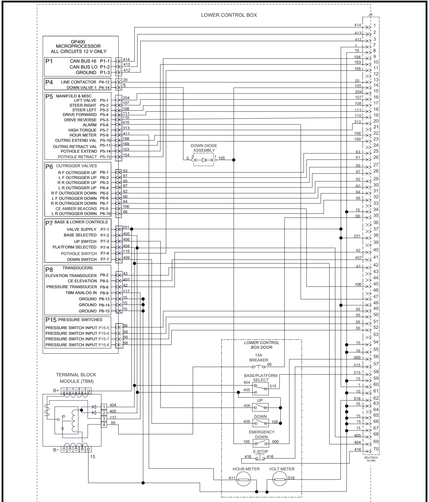
Figure 5-9: Electrical Schematic -- Later Machines, 1 of 3
