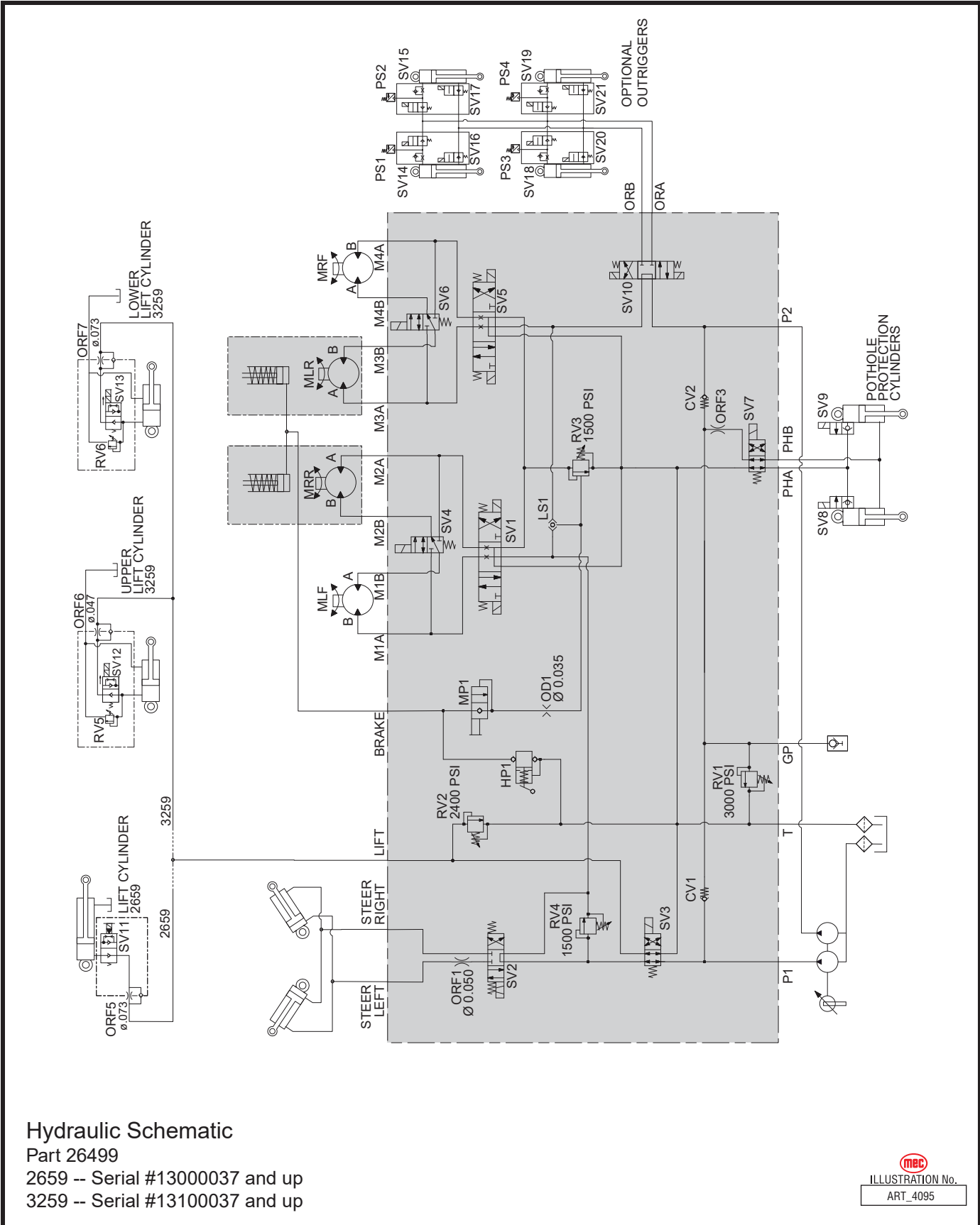
Figure 5-4: Hydraulic Schematic, Later Machines
