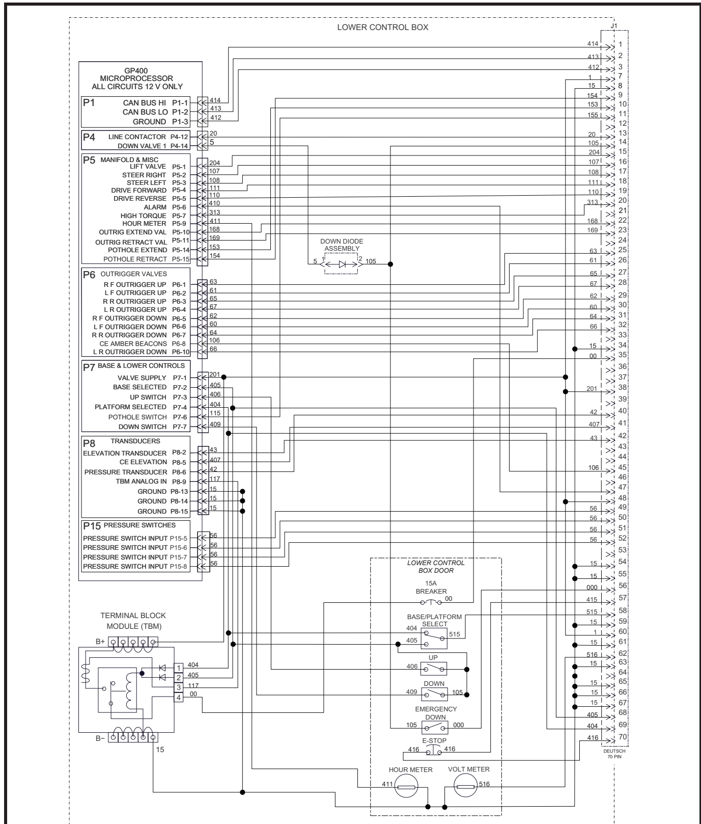
Figure 5-6: Electrical Schematic -- Early Machines, 1 of 3
