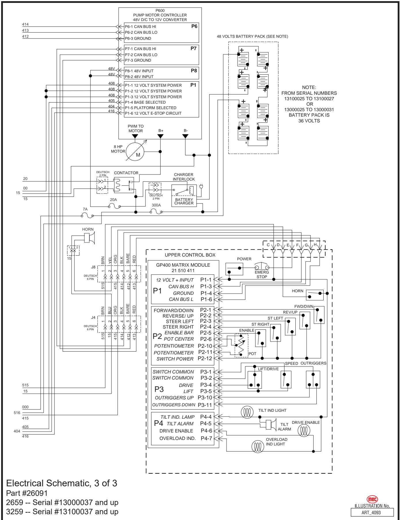
Figure 5-11: Electrical Schematic -- Later Machines, 3 of 3
