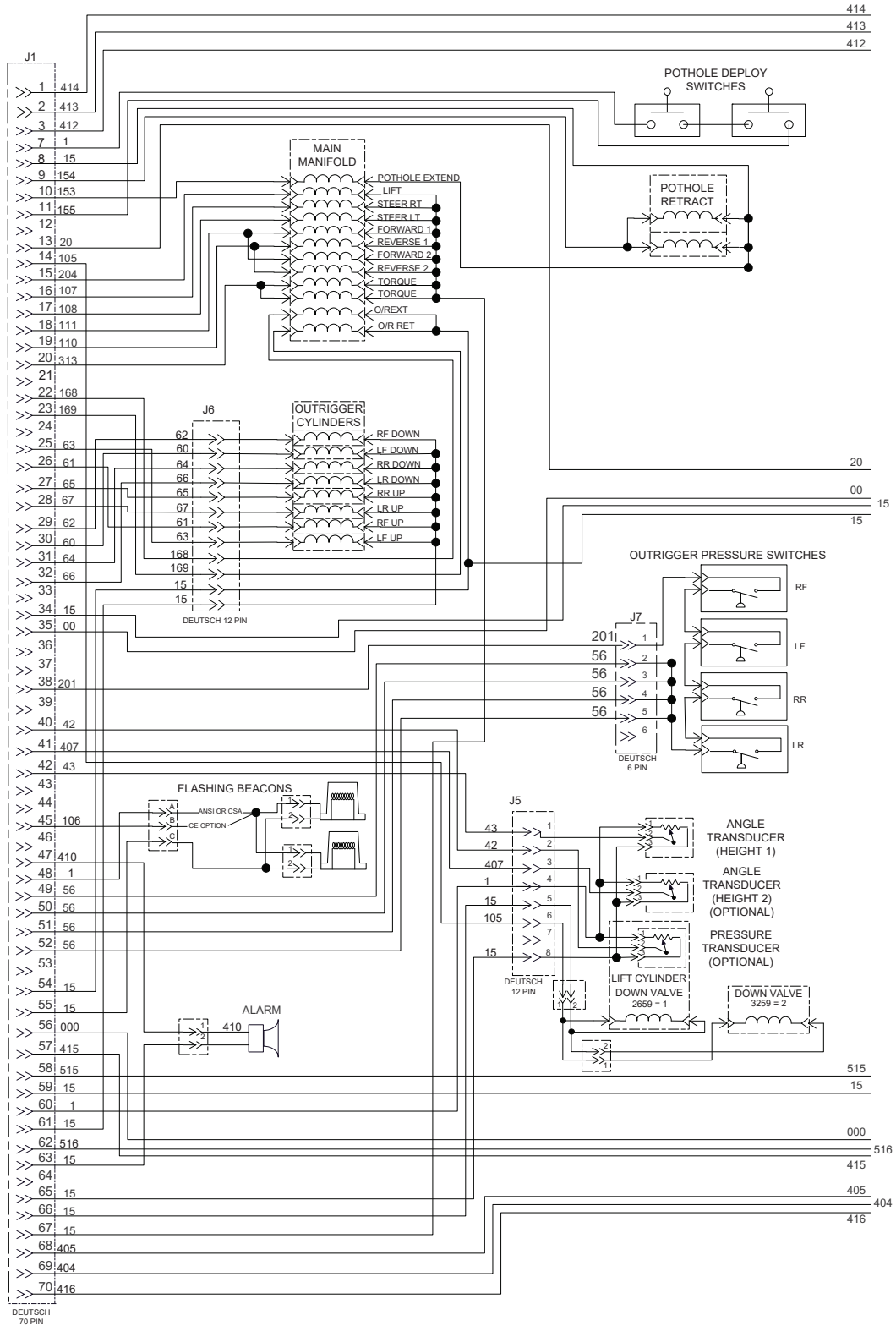
Electrical Schematic, 2 of 3 Part #26091 2659 -- Serial #1300037 and up 3259 -- Serial #1310037 and up
