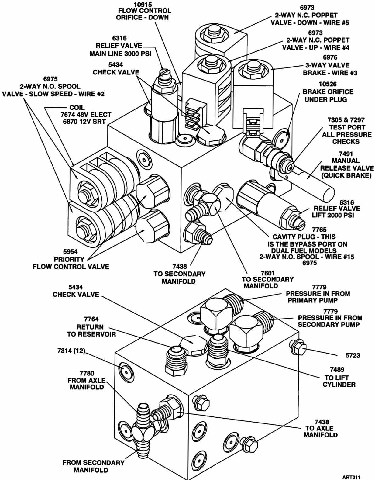
Figure 7-2. Primary Manifold
