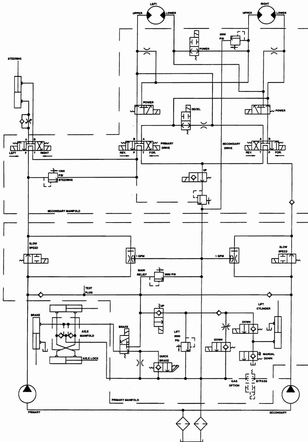
Figure 5-6. Quadrex Hydraulic Schematic
