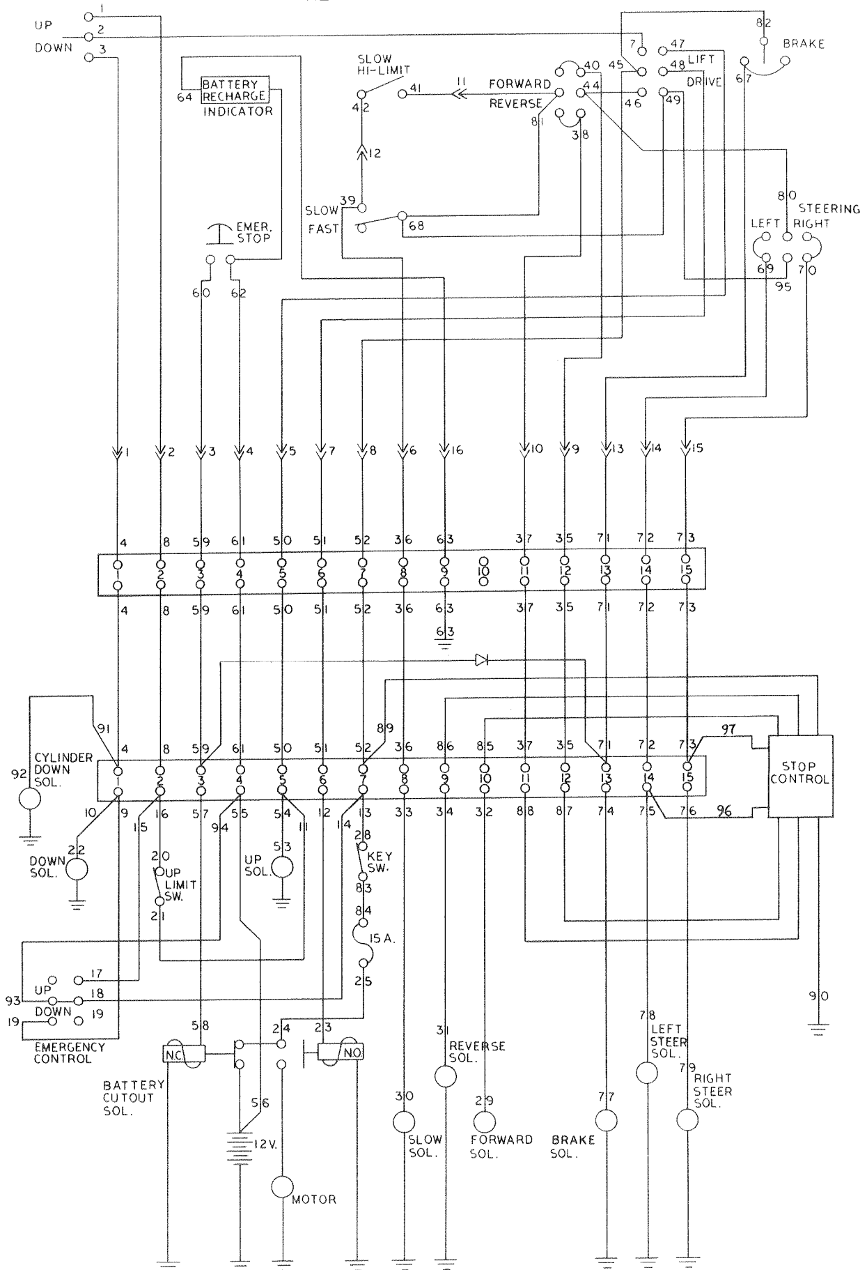
Figure 37. Wiring Diagram.
